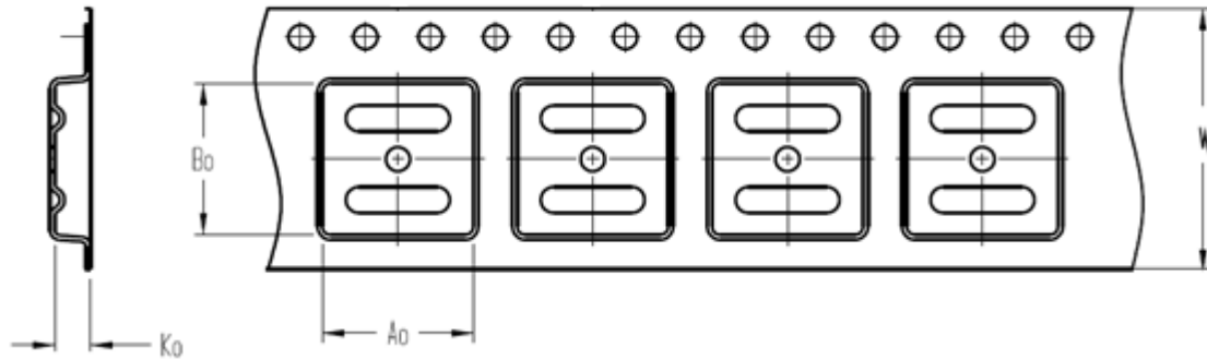
Figure. 28 Reel Packaging Specification
